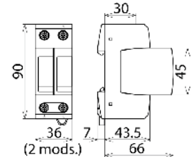
Dimension drawing DG M TT 2P 275
