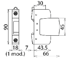
Dimension drawing DG S 600
