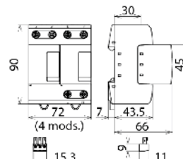
Dimension drawing DV M TT 2P 255 FM
