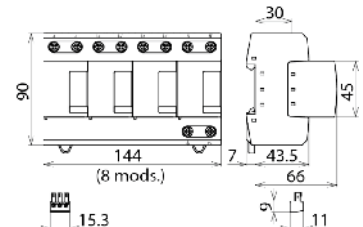
Dimension drawing DV M TT 255 FM
